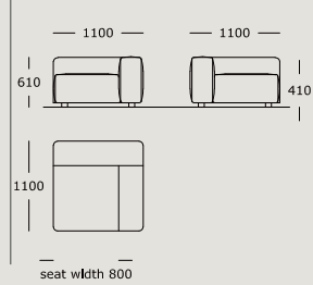
Module 21 Side/corner module right Back cushions not included
