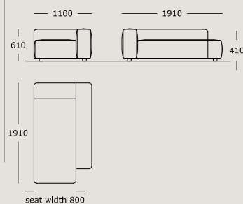
Module 14 Terminal, high arm, right Back cushions not included
