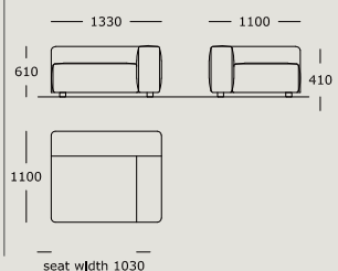
Module 10 Medium, high arm, right L Back cushions not included
