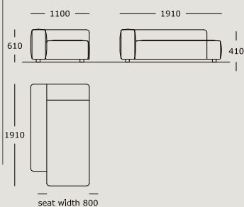
Module 13 Terminal, high arm, left Back cushions not included
