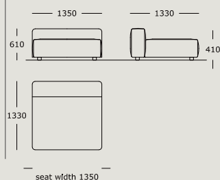
Module 15 Center, XL Back cushions not included
