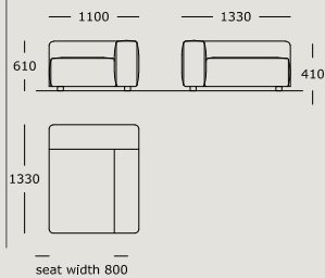
Module 5 Medium, high arm, left XL Back cushions not included
