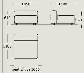
Module 20 Center Back cushions not included
