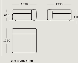
Module 9 Medium, high arm, left L Back cushions not included
