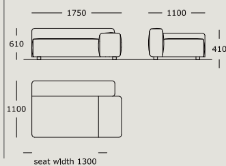
Module 8 Medium, low arm, right L Back cushions not included
