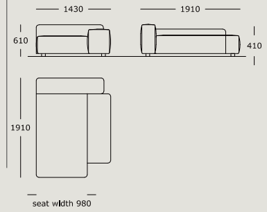
Module 21 Side/corner module right Back cushions not included
