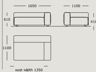
Module 12 Large, high arm, right L Back cushions not included
