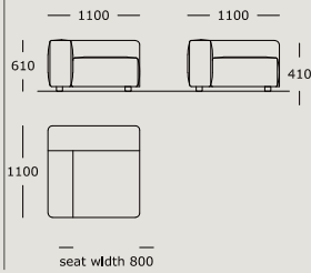
Module 19 Side/corner module left Back cushions not included
