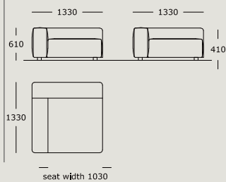
Module 8 Medium, low arm, right L Back cushions not included
