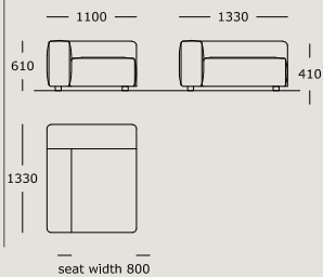
Module 4 Small, low arm, right L Back cushions not included
